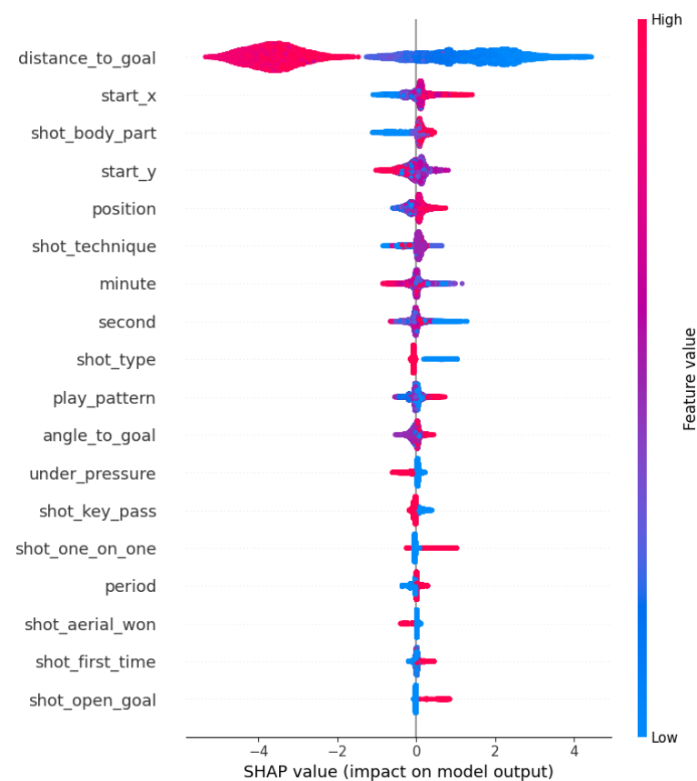
Gambar 4.27 Feature Importance
