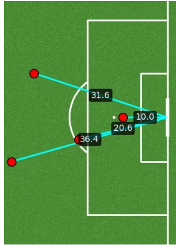
Gambar 4.19 Visualisasi distance_to_goal
